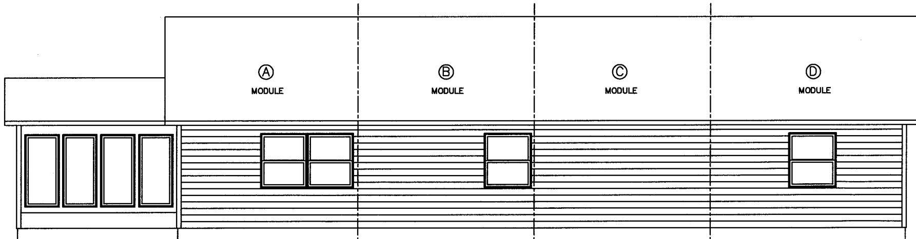
SIDE ELEVATION (2622 Sq.Ft.) 46x57 OFFICE.....52905
