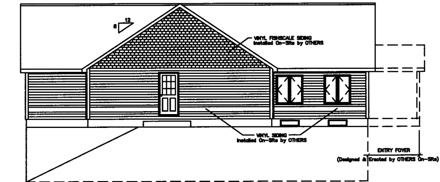
LEFT ELEVATION
