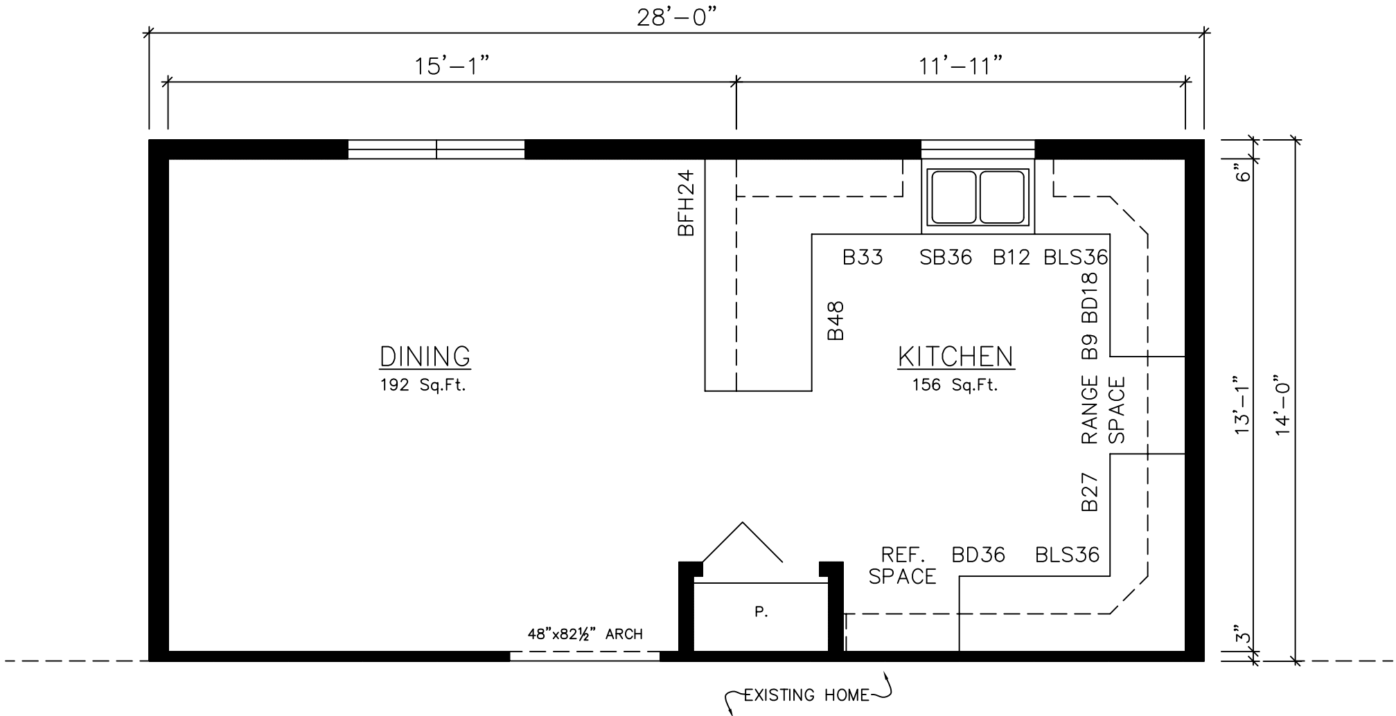
KITCHEN/DINING 22004 14'x28' (392 Sq. Ft.) Right Hand
