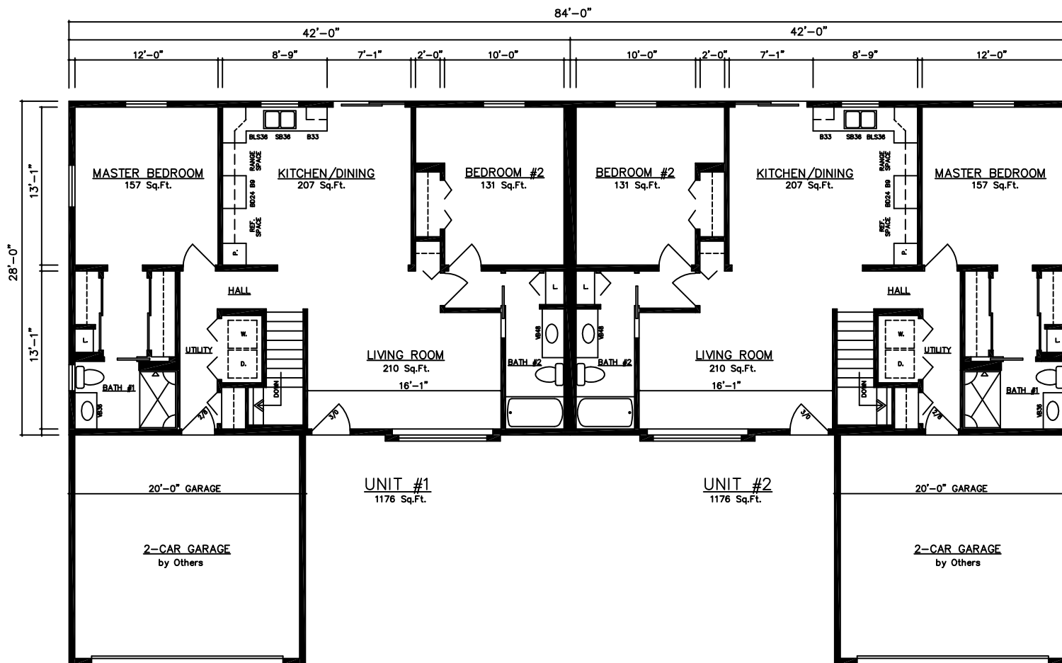
DUPLEX FLOOR PLAN
