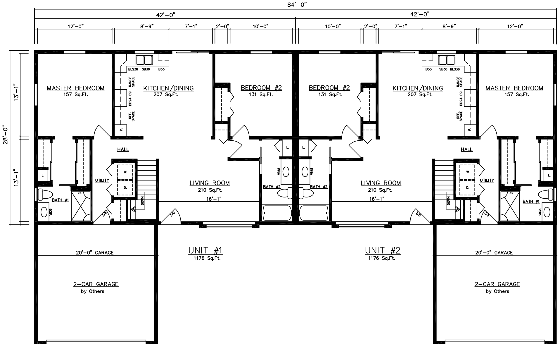
DUPLEX FLOOR PLAN
