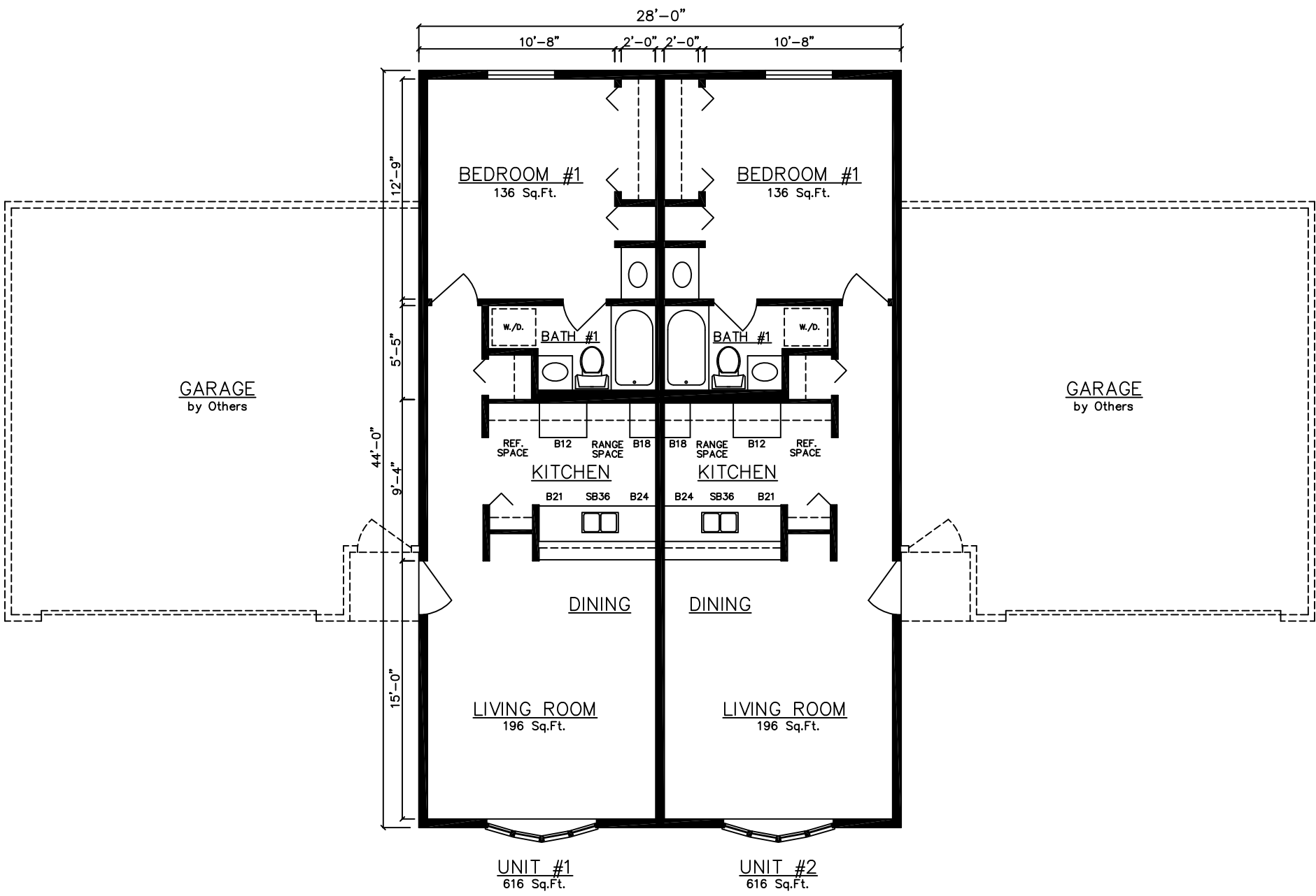
FLOOR PLAN AUBURN DUPLEX.....10105
