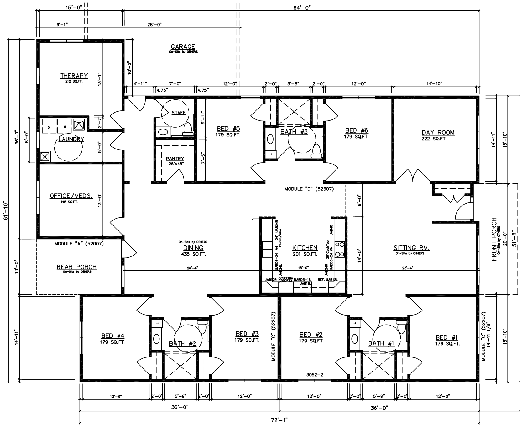
FLOOR PLAN 4013 TOTAL Sq.Ft.
