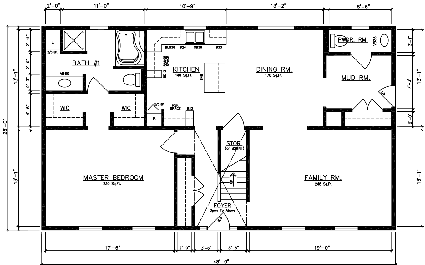
NORTHVILLE 14066...(Basement) (2,688 Sq.Ft.)
