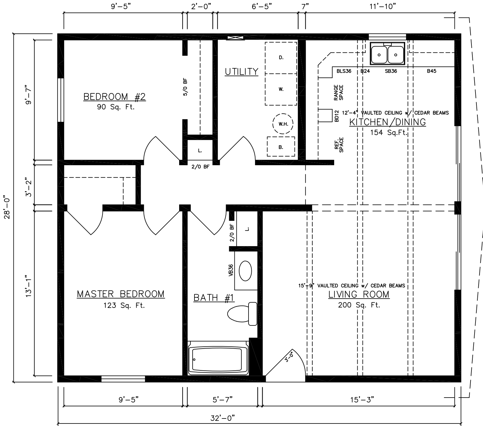
ALPINE 10510.....(Crawlspace) 28'x32' (896 Sq.Ft.) 2 Bed, 1 Bath
