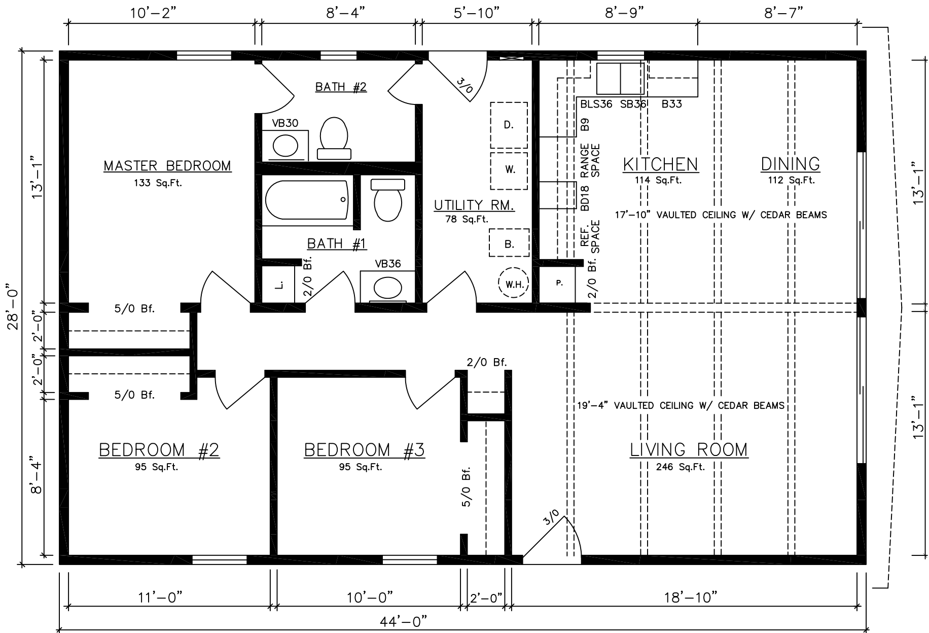
ALPINE 10602...(Crawlspace) 28'x44' (1,232 Sq.Ft.) 3 Bed, 1½ Bath
