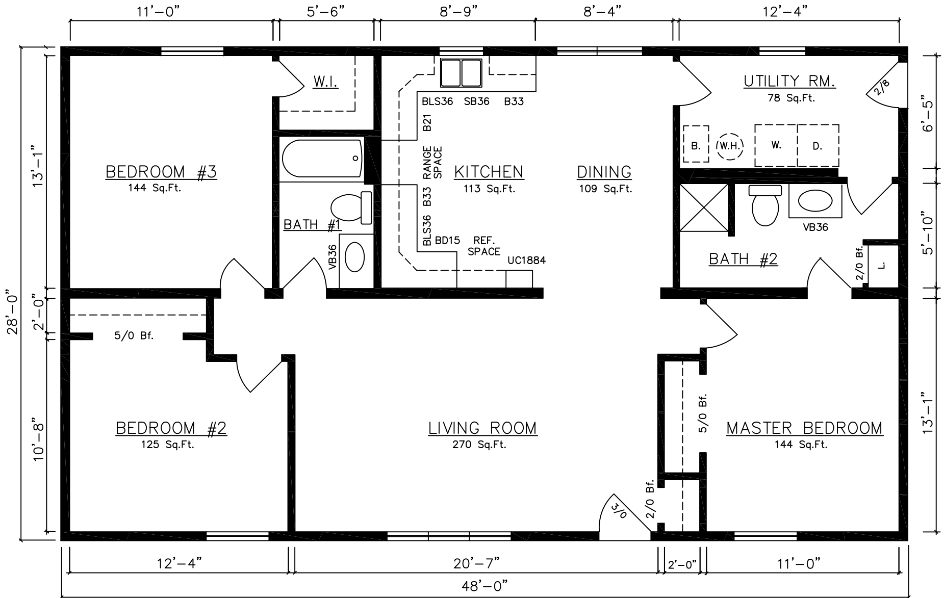
AMHERST 10402...(Crawlspace) 28'x48' (1,344 Sq.Ft.) 3 Bed, 1 3/4 Bath
