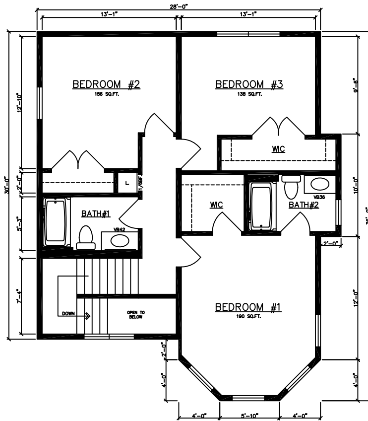
BAYVIEW 16024 (CRAWLSPACE) (1856 Total Sq.Ft.) 3 Bed, 2-1/2 Bath SECOND FLOOR PLAN (928 Sq.Ft.)
