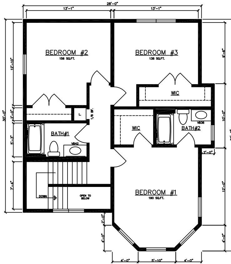
BAYVIEW 16026 (BASEMENT) (1856 Total Sq.Ft.) 3 Bed, 2-1/2 Bath SECOND FLOOR PLAN (928 Sq.Ft.)
