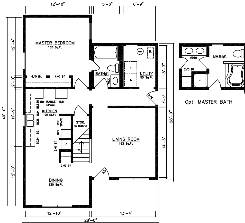
BRECKENRIDGE 13102...(Basement) (1,512 Sq.Ft.) 3 Bed, 2 Bath
