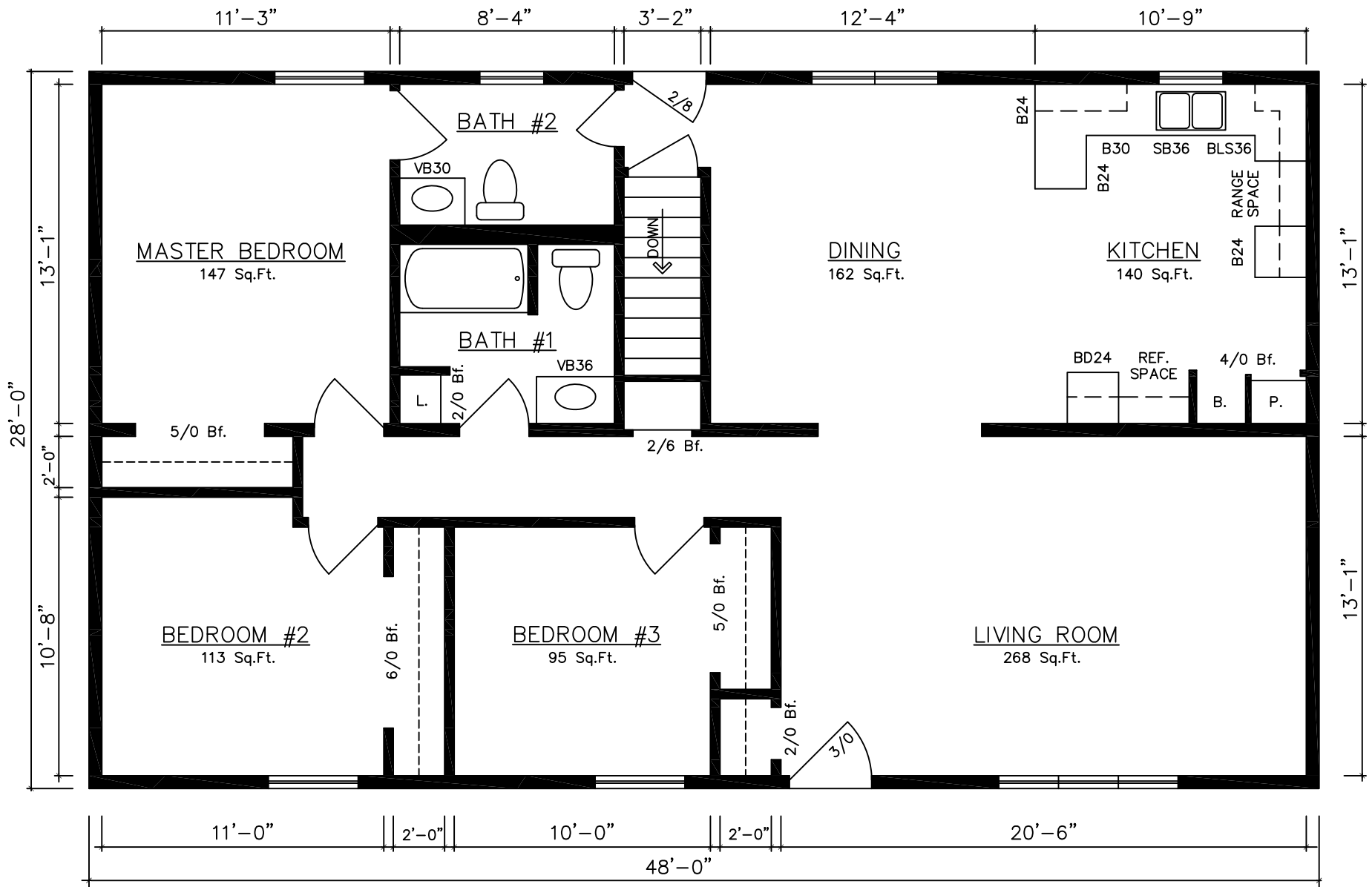
BRISTOL 10304...(Basement) 28'x48' (1,344 Sq.Ft.) 3 Bed, 1½ Bath
