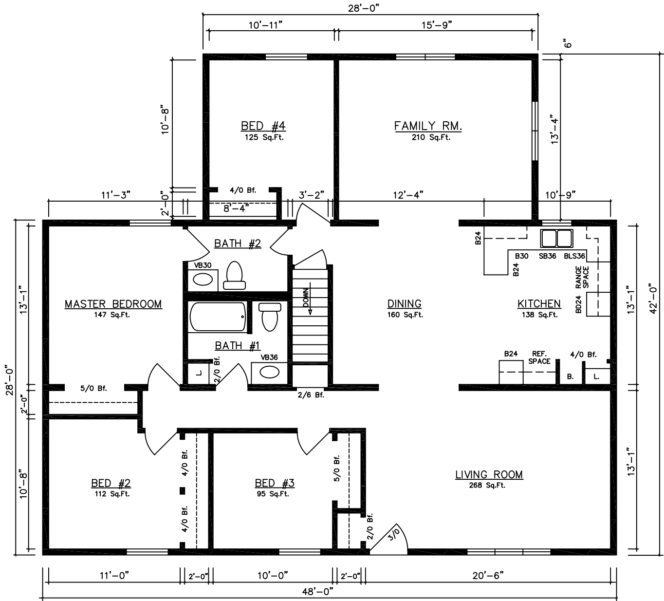
BRISTOL 10311...(Basement) 48' (1,736 Sq.Ft.) 4 Bed, 1-3/4 Bath
