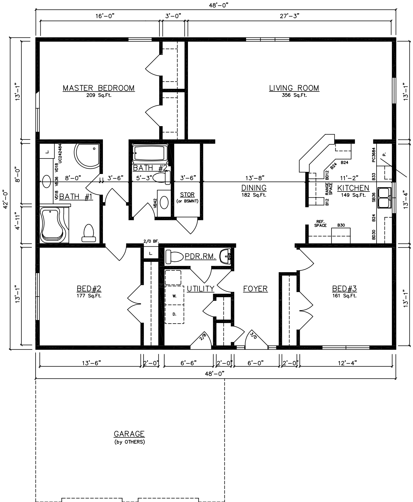
CLARKSTON 14122...(Basement) 42'x48' (2,016 Sq.Ft.) 3 Bed, 2½ Bath
