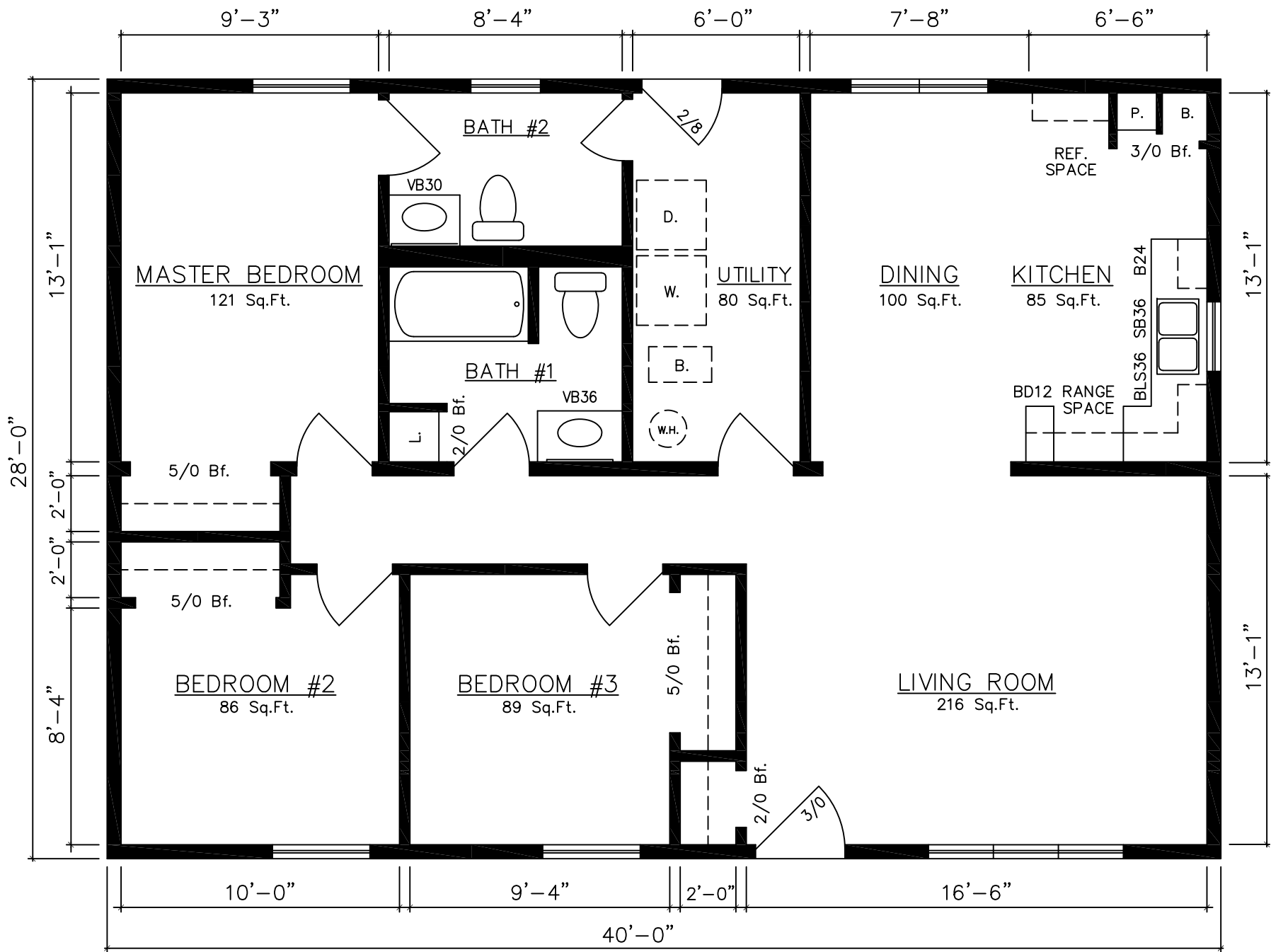
DANBURY 10102...(Crawlspace) 28'x40' (1,120 Sq.Ft.) 3 Bed, 1½ Bath
