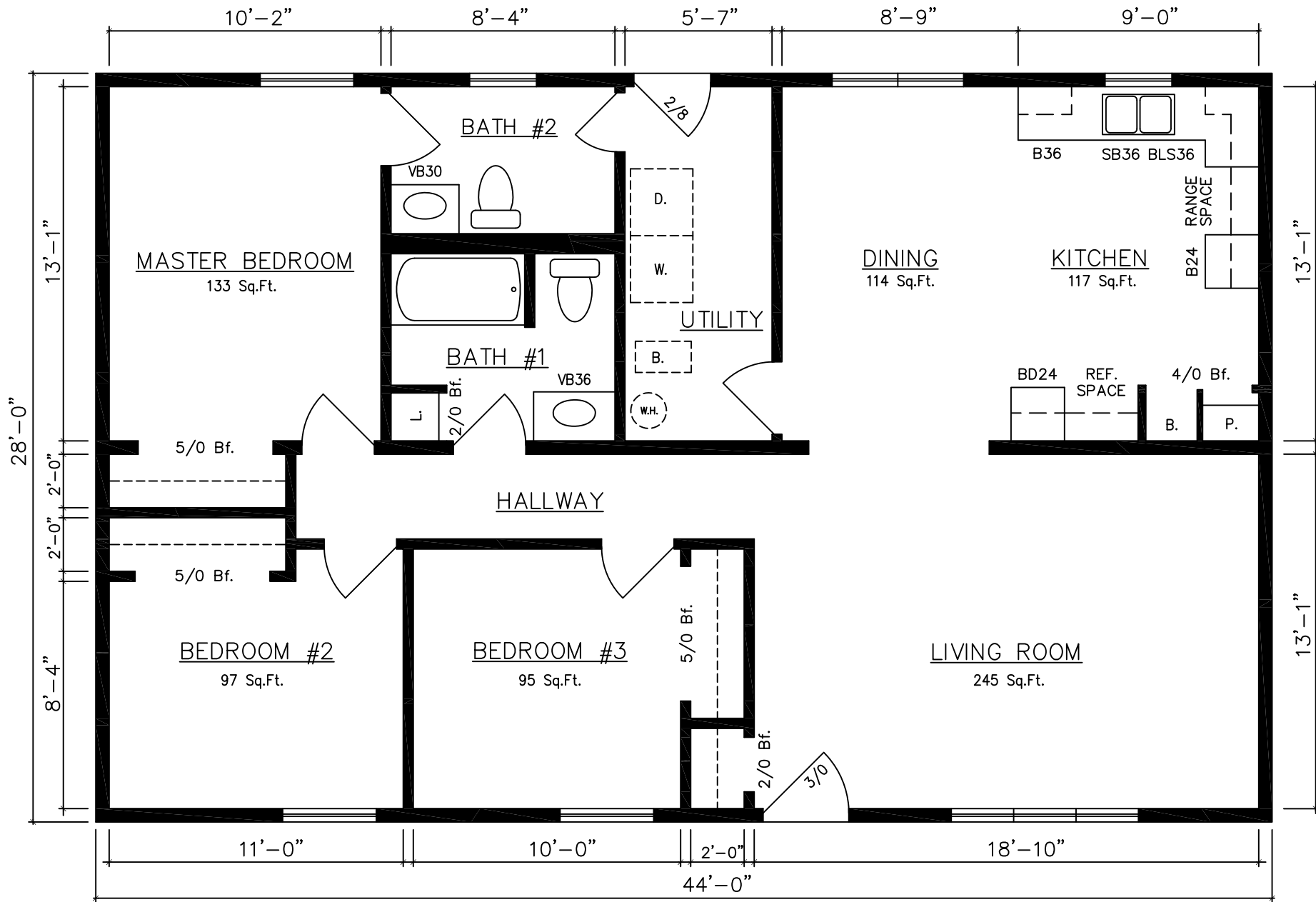
HAMDEN 10202...(Crawlspace) 28'x44' (1,232 Sq.Ft.) 3 Bed, 1½ Bath
