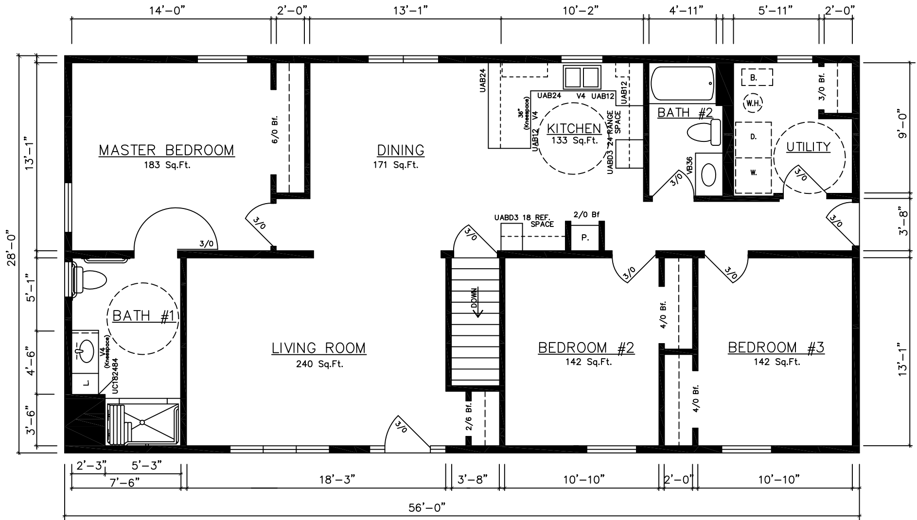
NORTHPORT 10492UA...(Basement) 28'x56' (1568 Sq.Ft.) 3 Bed, 2 Bath Universal Access
