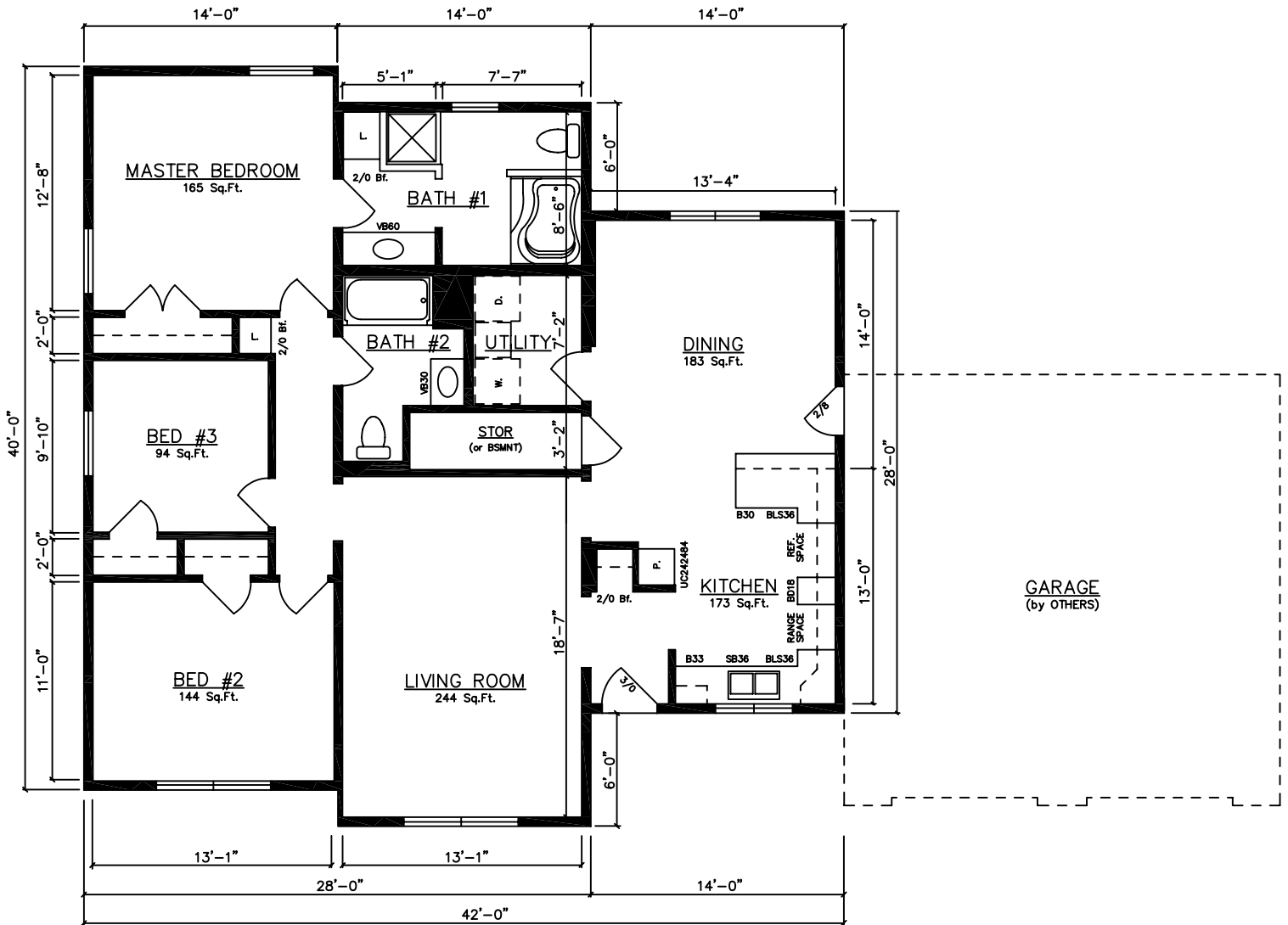
RICHVILLE 12224...(Crawlspace)40' (1,512 Sq.Ft.) 3 Bed, 2 Bath
