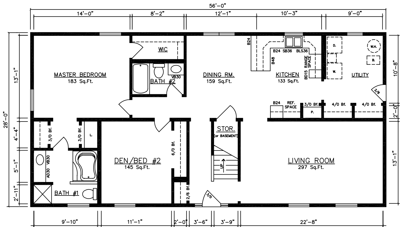
WILLIAMSBURG 10050...(Basement) 28'x56' (2,594 Sq.Ft.)
