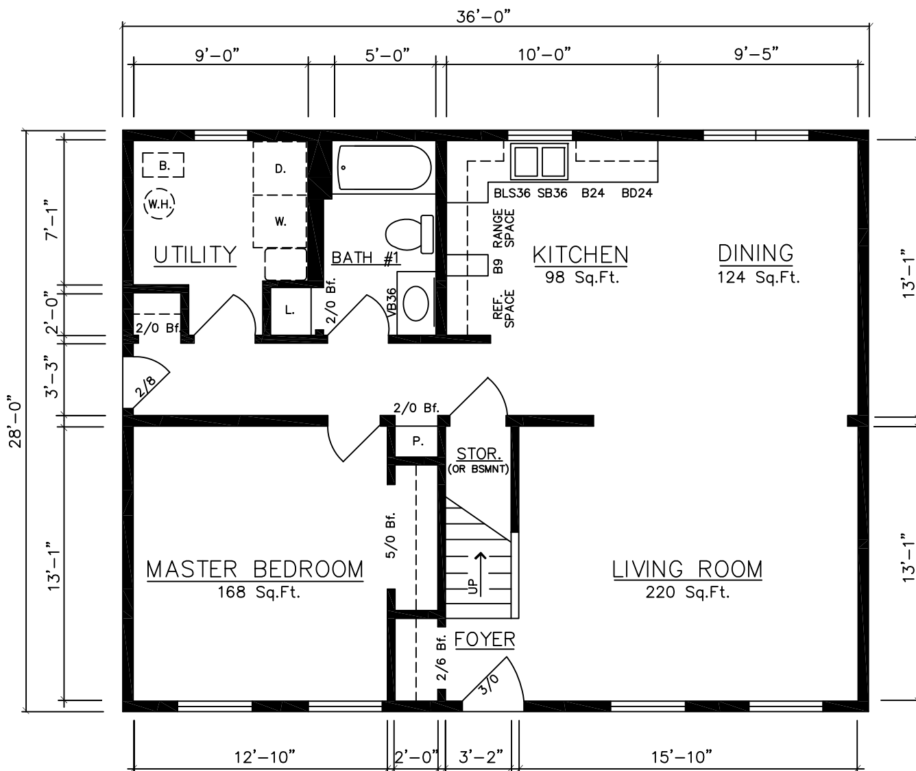
WILLIAMSBURG 11016...(Basement) 28'x36' (1,668 Sq.Ft.)
