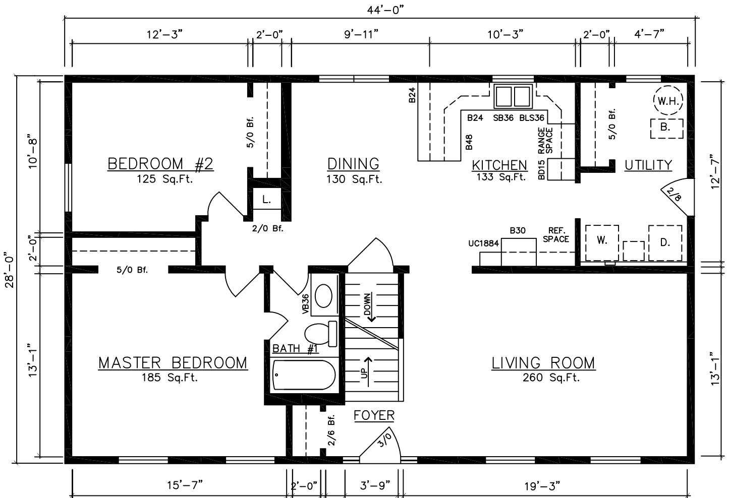
WILLIAMSBURG 11160...(Basement) 28'x44' (2,038 Sq.Ft.)
