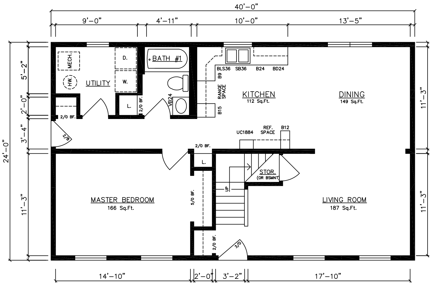
WILLIAMSBURG 24042...(Basement) 24'x40' (1,627 Sq.Ft.)
