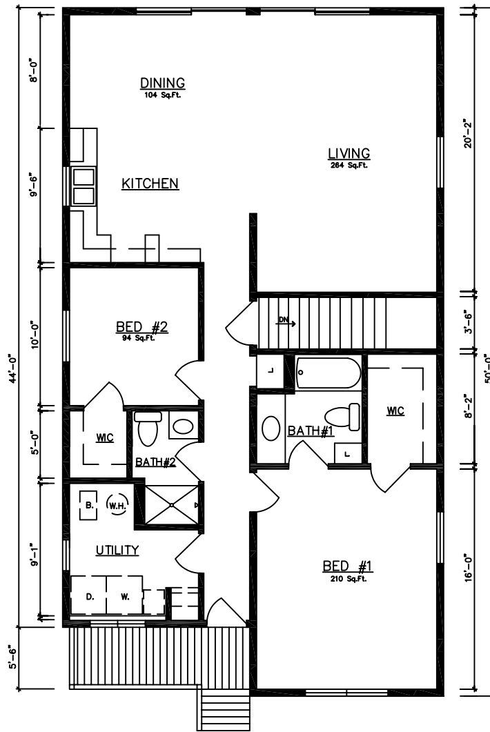
FLOOR PLAN ALPINE ...10526 1316 Sq.Ft.
