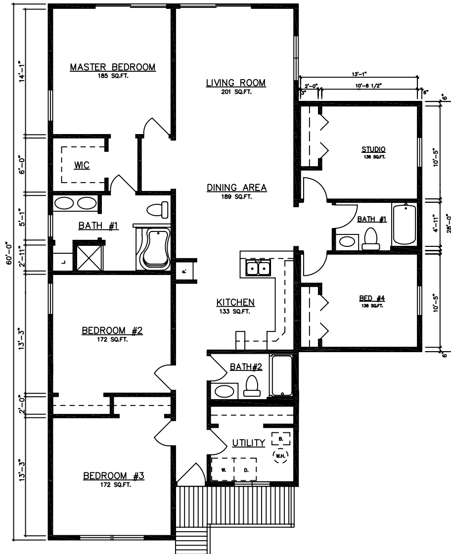
FLOOR PLAN 1988 Sq.Ft.
