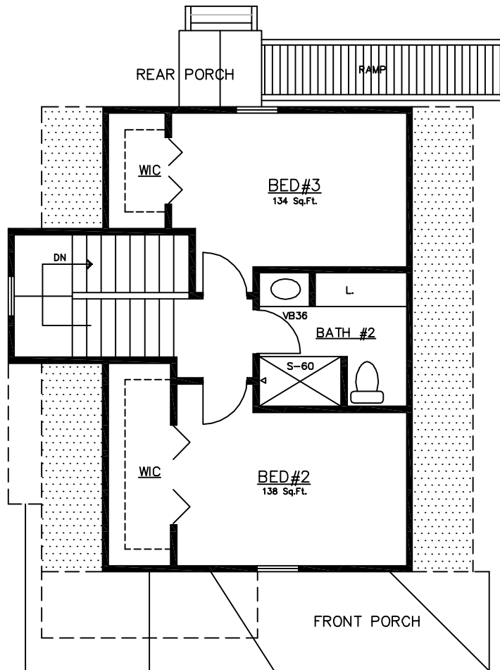
2nd..Fl. PLAN 780 Sq.Ft.(1st) + 320 Sq.Ft.(2nd) 1100 Sq.Ft. TOTAL
