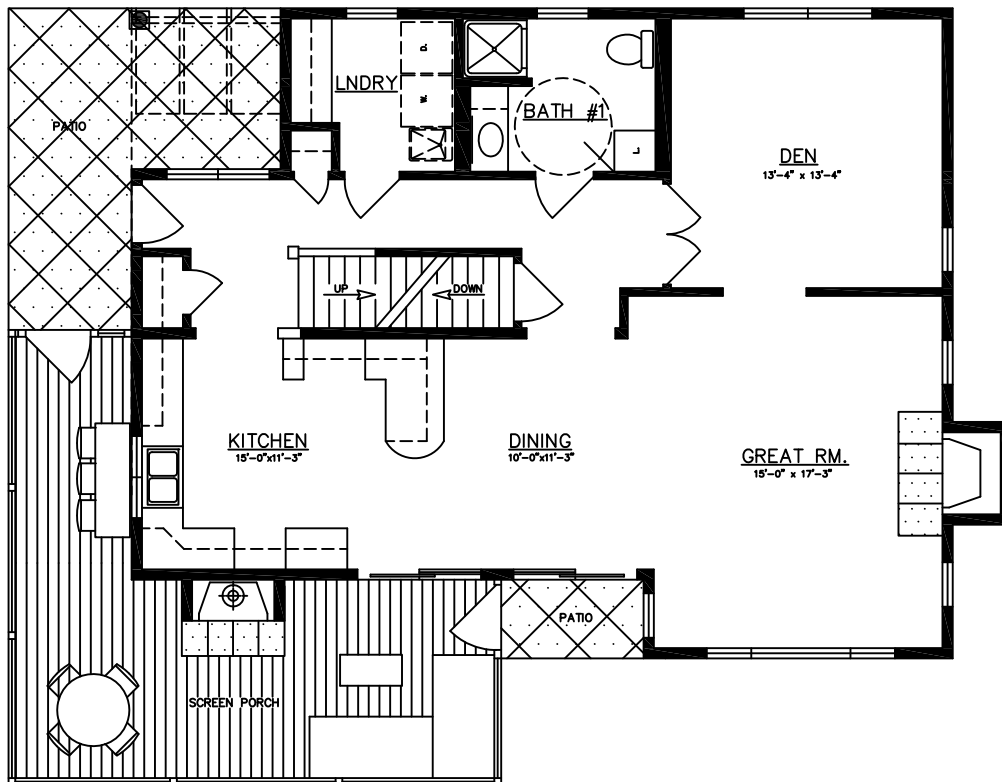
FIRST FLOOR PLAN (BASEMENT)
