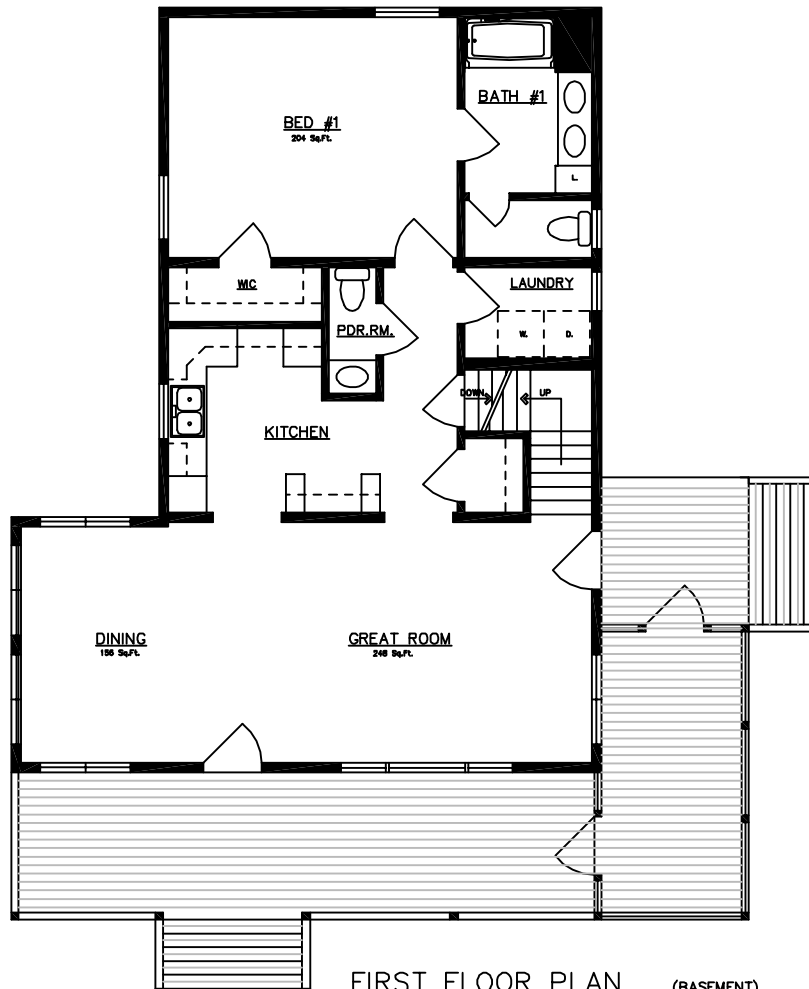
FIRST FLOOR PLAN (BASEMENT)
