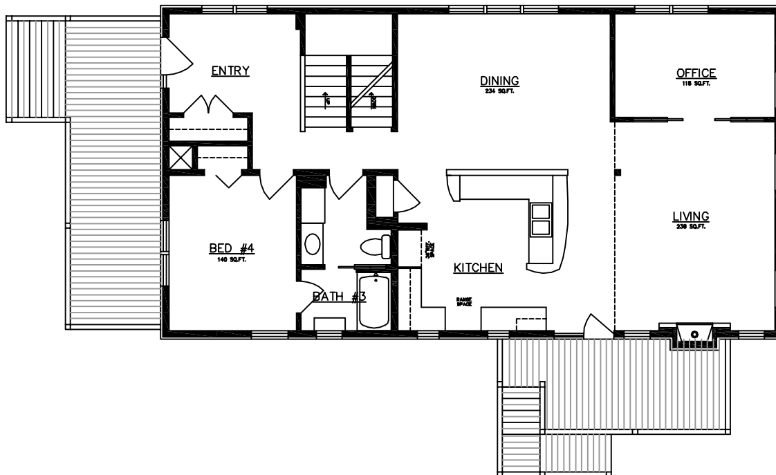
FIRST FLOOR PLAN (BASEMENT)
