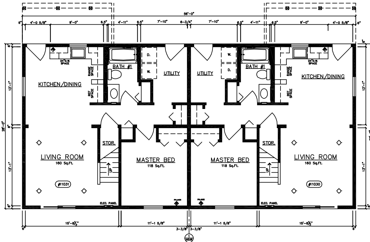
1st.FI. PLAN (CRAWLSPACE)
