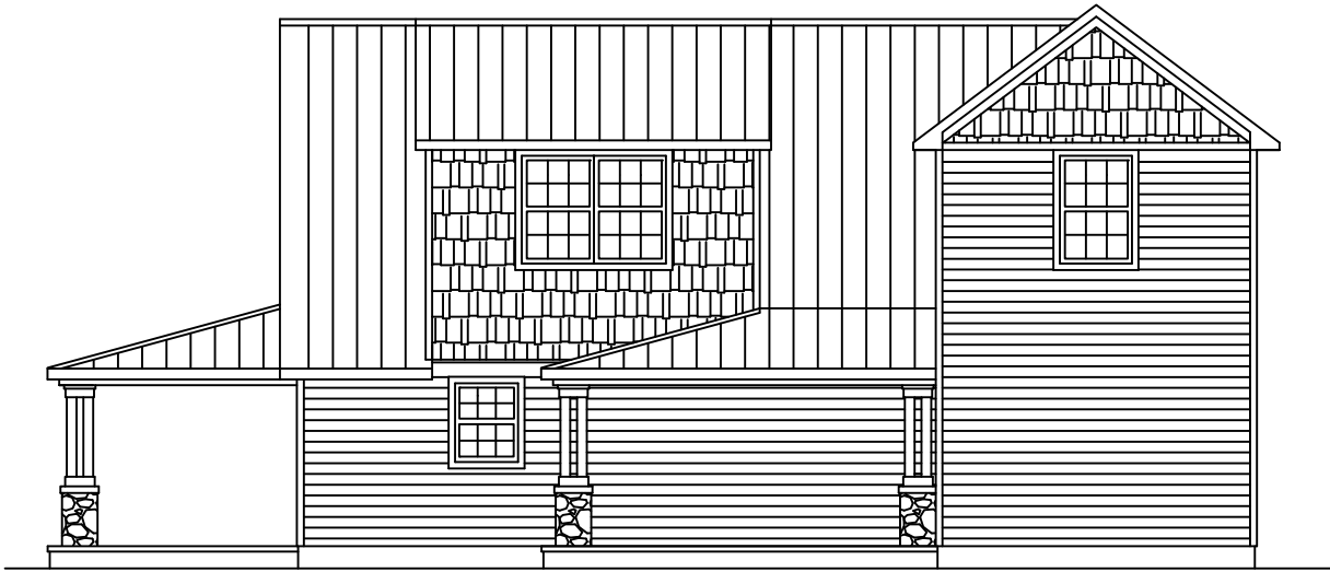
REAR ELEVATION
