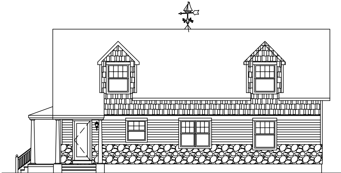
STREET ELEVATION
