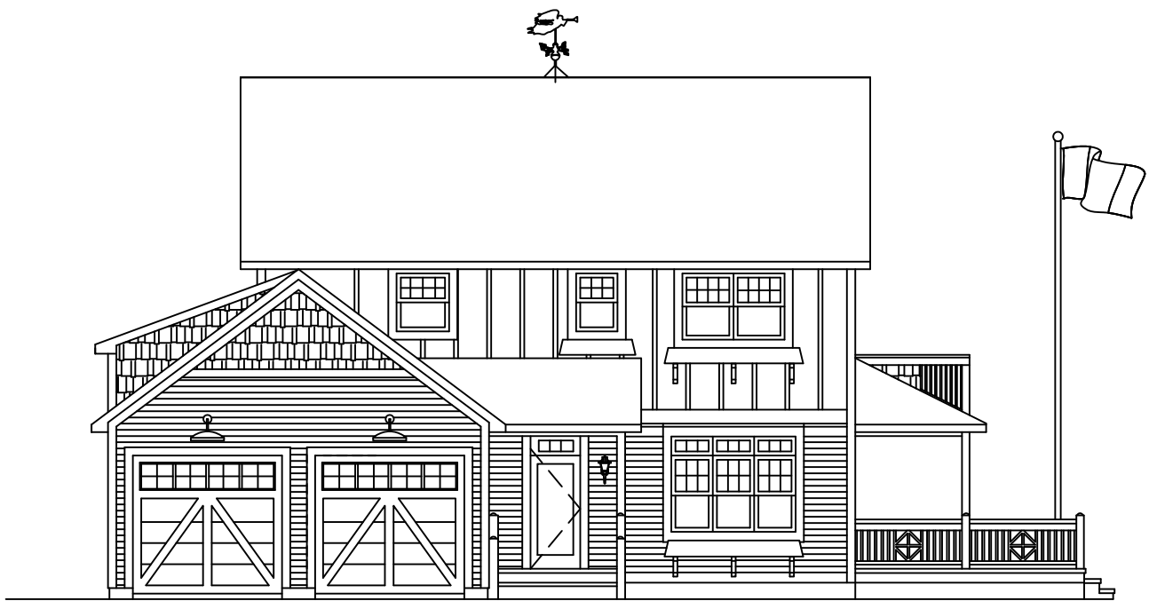
STREET ELEVATION
